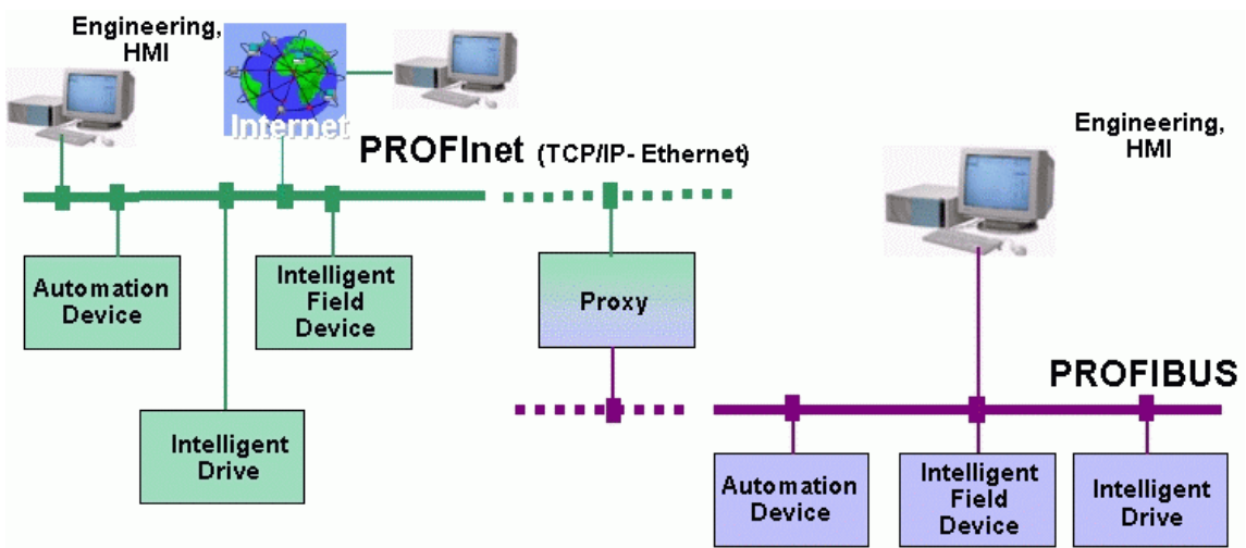
The vertical expansion of the tried and tested PROFIBUS technology
