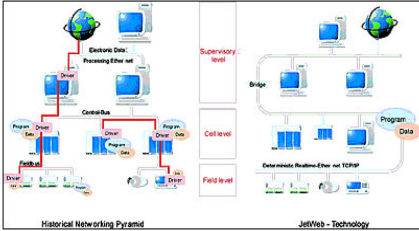
Historical Networking Pyramid
