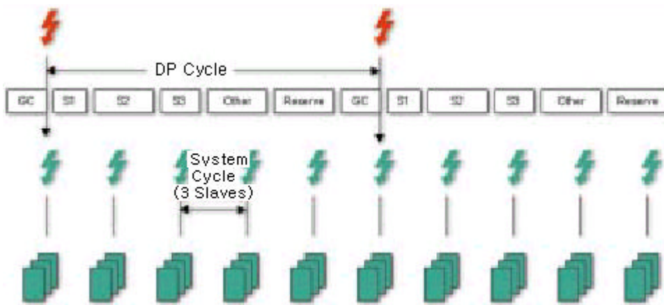
4. MC solution based on PROFIBUS
